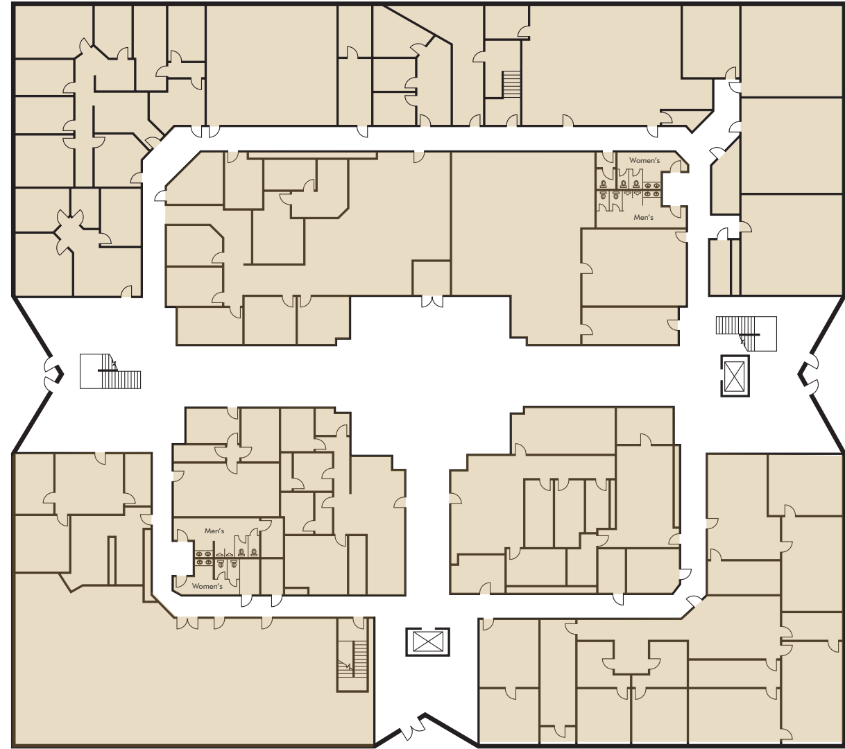
FIRST FLOOR
